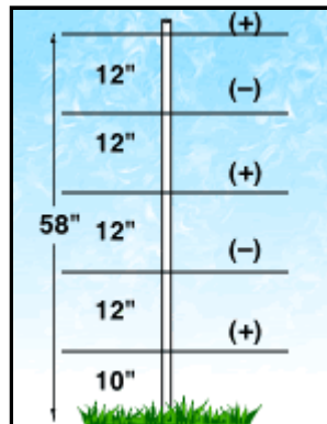
Beef or Dairy Cattle 5 foot high - 5 wire
