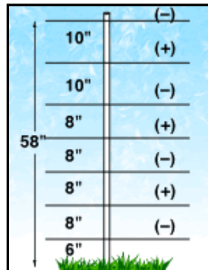
Beef or Dairy Cattle 5 foot high - 7 wire
