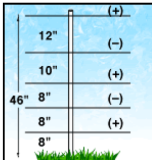
Beef or Dairy Cattle 4 foot high - 5 wire
